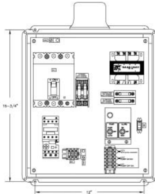
Model #S463 w/Audible PIEZO AUDIBLE WILL BE MOUNTED THROUGH THE BOTTOM OF THE ENCLOSURE. BELL OR HORN WILL BE MOUNTED ON THE RIGHT-SIDE OF THE ENCLOSURE.
